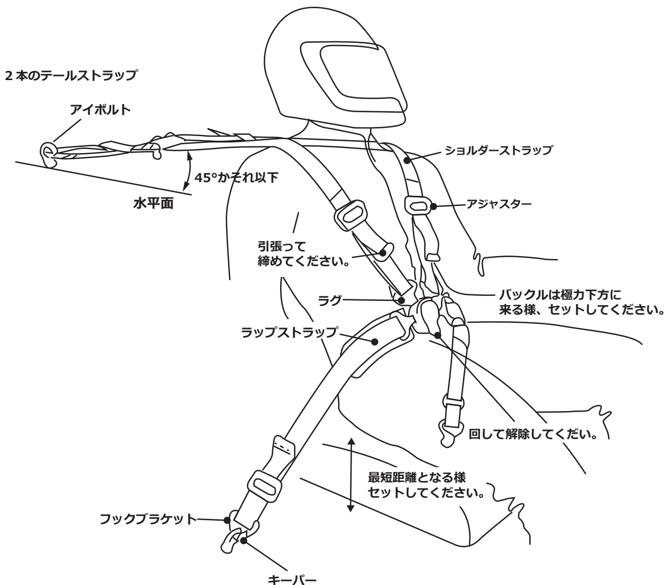
Fig 1- 全体構成図 -CLUB4 (FOR 2SEATER SPORTS VEHICLE)
